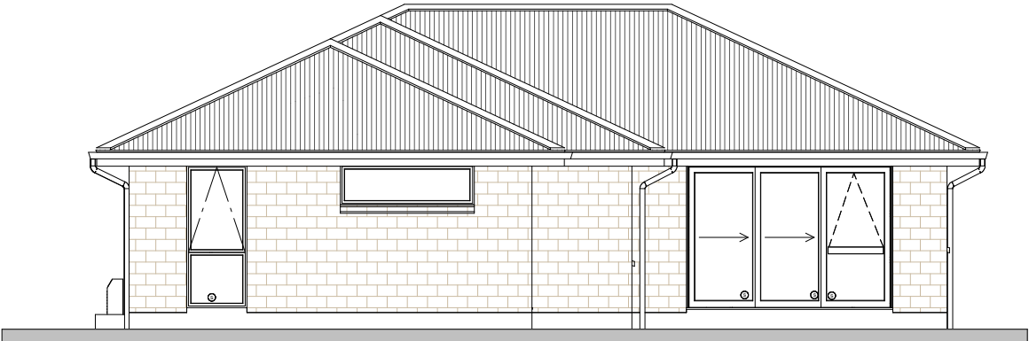
East Elevation
