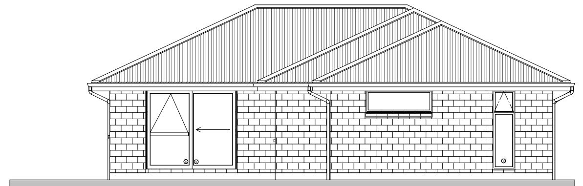
West Elevation
