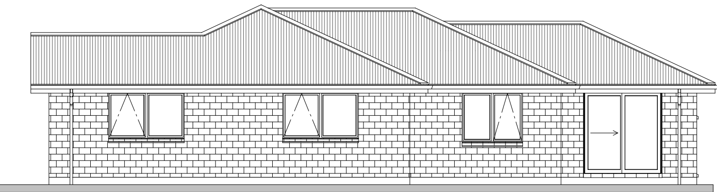
North Elevation
