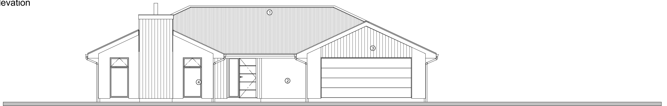
West Elevation
