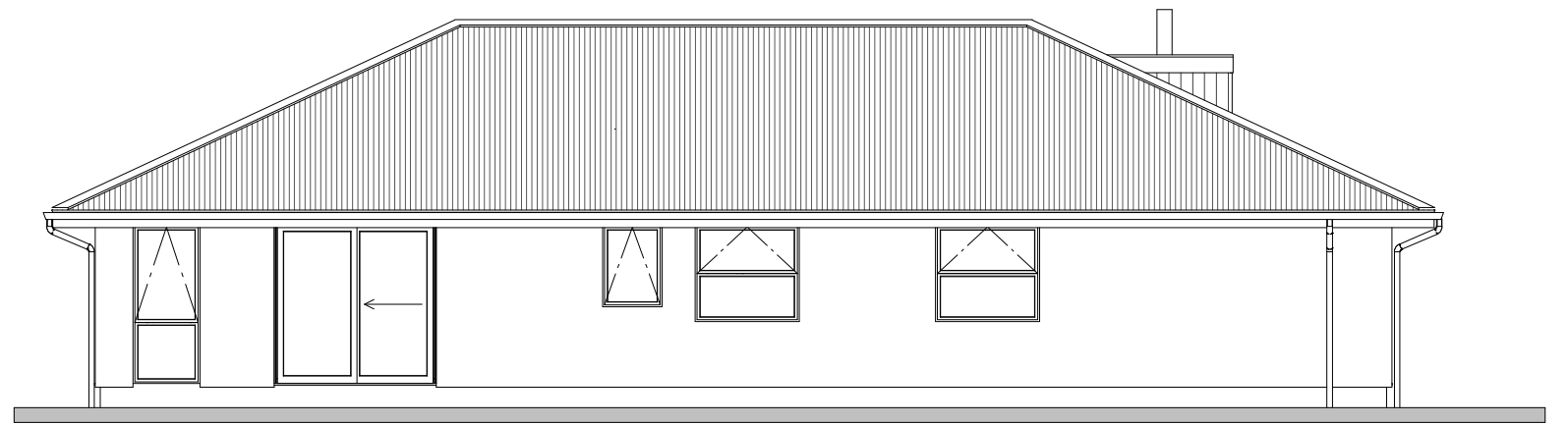
East Elevation
